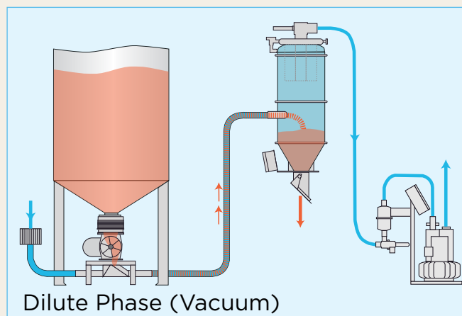
Series 2400 receiver conveying salt
